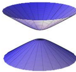
Hyperboloid of two sheets
