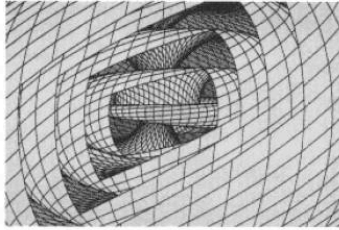
Fig. 3.6 The patterns in a three-dimensional BZ mixture are more complex. One of the simplest, the analogue of a two-dimensional spiral, is the scroll wave (a), which can curl up on itself to form a scroll ring. Twisted scroll rings have more complicated structures (b). (Images: Arthur Winfree, University of Arizona.)
