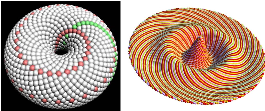
Below: Left, torus centrifugal flow around a disk magnet, right magnetic pressure gradients with high pressures showing raised, not to scale. This same pattern on the right is reproduced in electrification of the dielectric inertial plane against a magnetic field over time.
