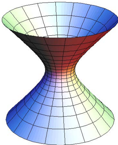
Hyperboloid of one sheet
