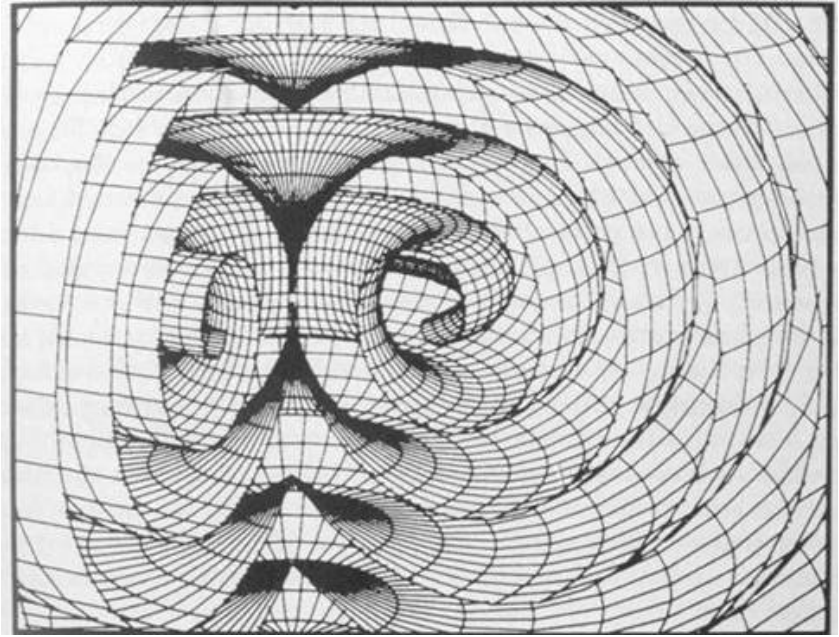
Fig. 3.6 The patterns in a three-dimensional BZ mixture are more complex. One of the simplest, the analogue of a two-dimensional spiral, is the scroll wave (a), which can curl up on itself to form a scroll ring. Twisted scroll rings have more complicated structures (b). (Images: Arthur Winfree, University of Arizona.)
